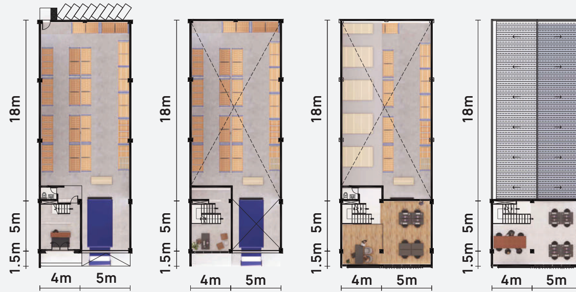
DENAH LANTAI 1
