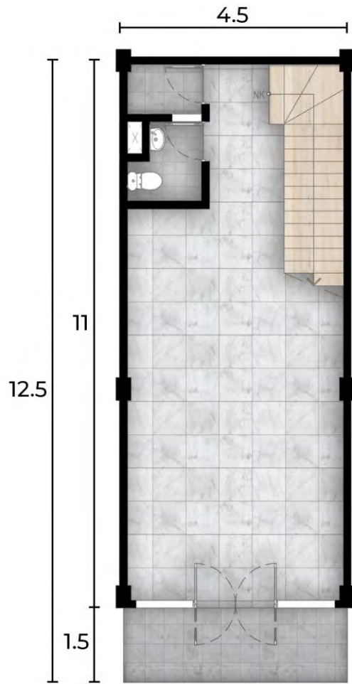
LANTAI 1
