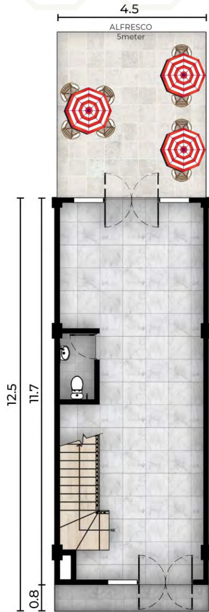
LANTAI 1
